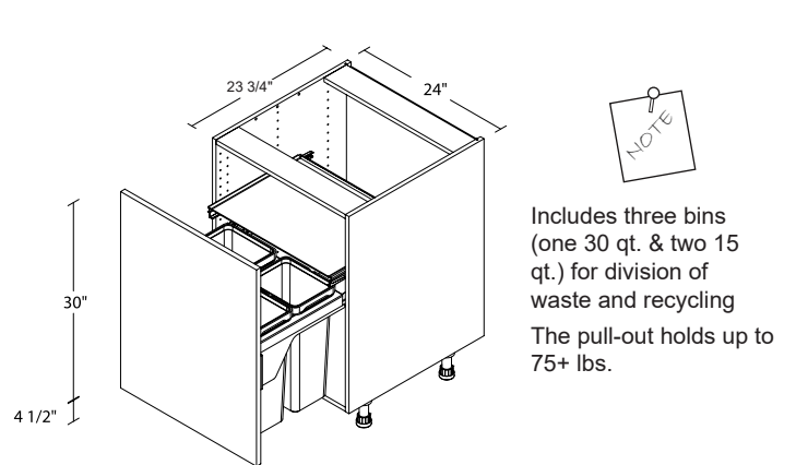
BASE PULL-OUT WITH 3 WASTE BINS / FULL-HEIGHT DOOR 24" B24FHSWB
