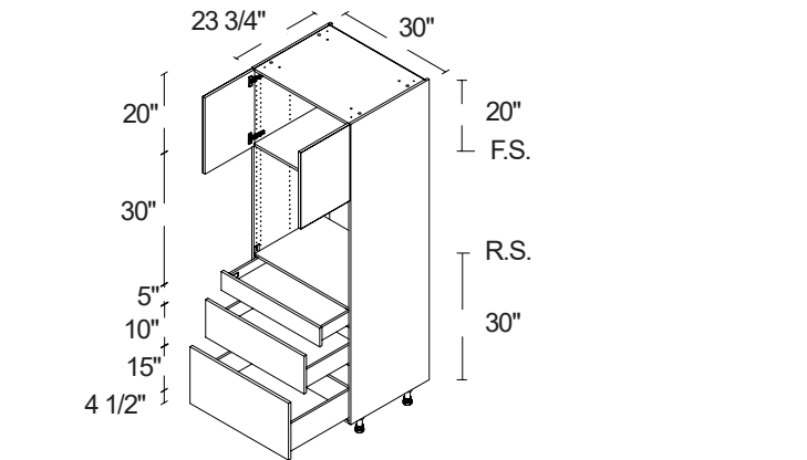
TALL SINGLE OVEN 4 / 2 DOORS / 3 DRAWERS
