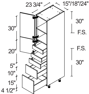
TALL 4 DOORS / 3 DRAWERS / 2 INNER DRAWERS
