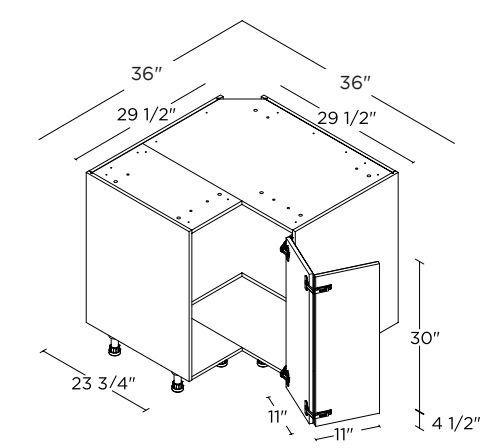
CORNER BASE WITH DURABLE POLYMER LAZY SUSAN 36" BC36LS(L/R)
