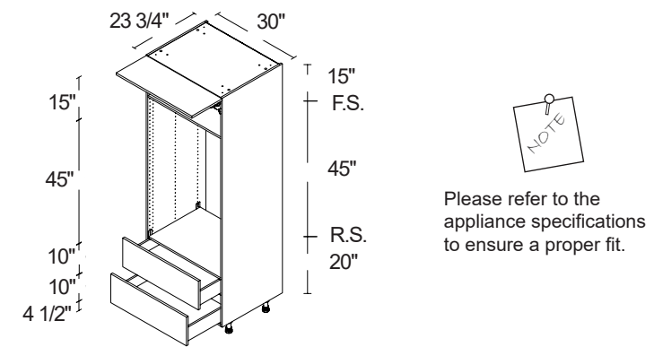
TALL MICRO / WALL OVEN 3 / 1 LIFT-UP DOOR / 2 DRAWERS
