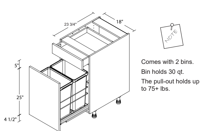
BASE PULL-OUT WITH 2 WASTE BINS / 1 DRAWER 18" B18SWB
