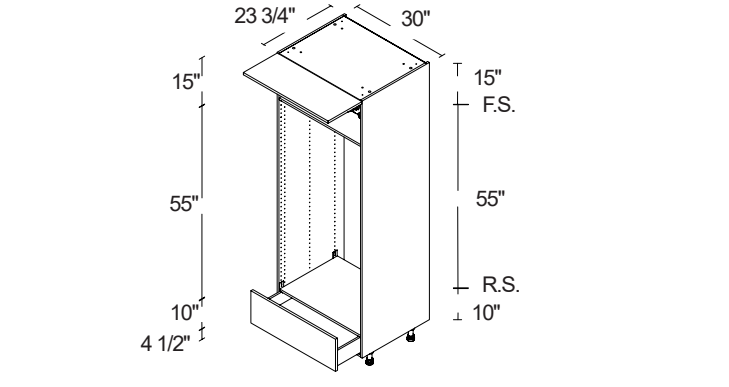
TALL DOUBLE OVEN 3 / 1 LIFT-UP DOOR / 1 DRAWER
