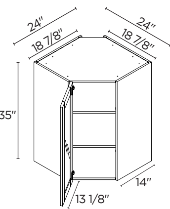
CORNER WALL 35" HIGH / 1 GLASS DOOR*
