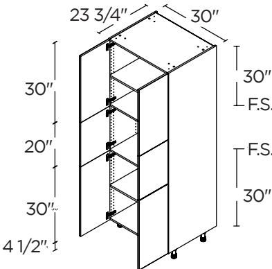
TALL 6 DOORS
