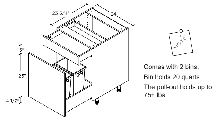
BASE PULL-OUT WITH 2 WASTE BINS / 1 DRAWER 24" BPO24
