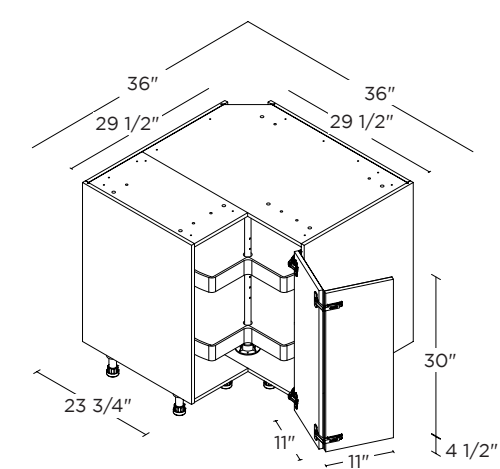
CORNER BASE WITH PREMIUM LAZY SUSAN 36" BC36LSP(L/R)
