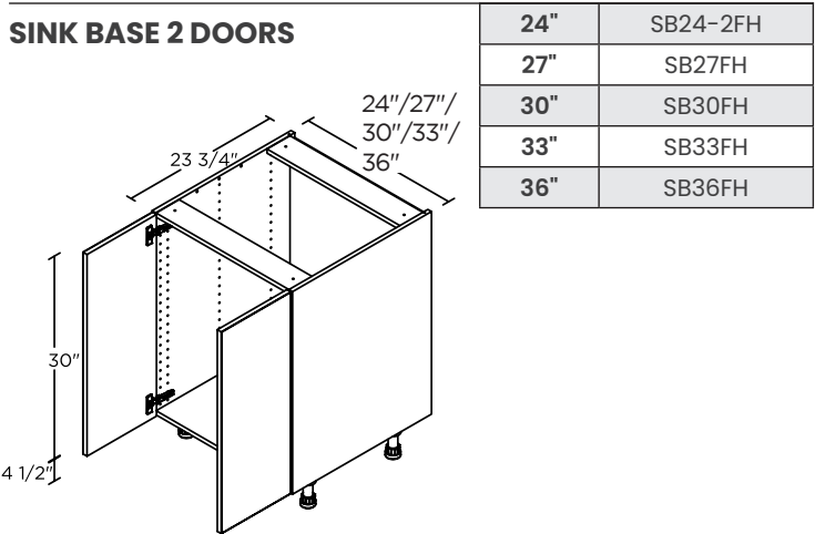
SINK BASE 2 DOORS / 1 FIXED FRONT
