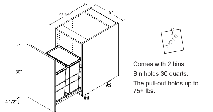
BASE PULL-OUT WITH 2 WASTE BINS / FULL-HEIGHT DOOR 18" B18FHSWB
