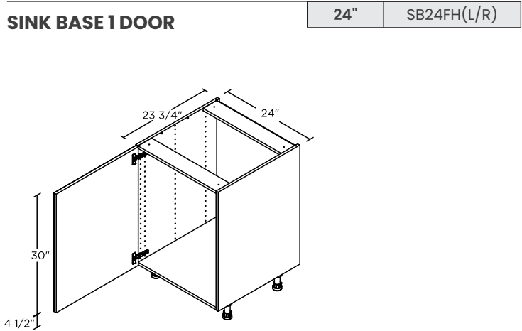
SINK BASE 1 DOOR / 1 FIXED FRONT
