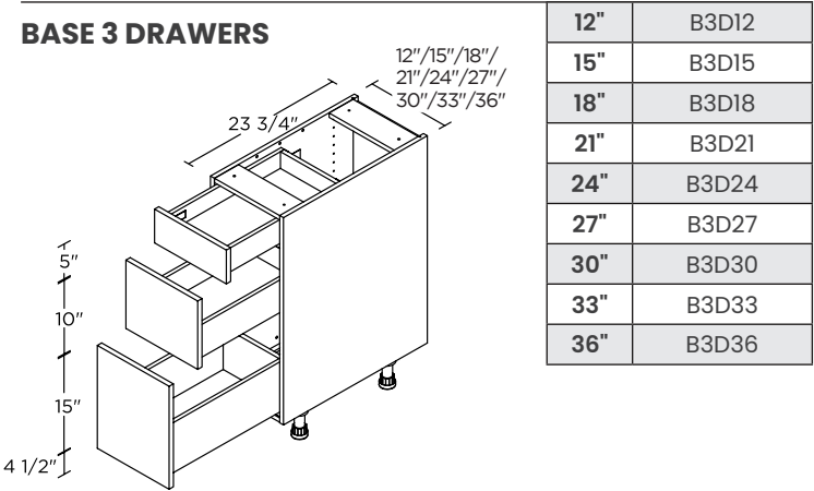
BASE 3 DRAWERS
