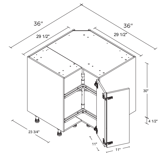
CORNER BASE WITH PREMIUM LAZY SUSAN 36" BC36LSP(L/R)
