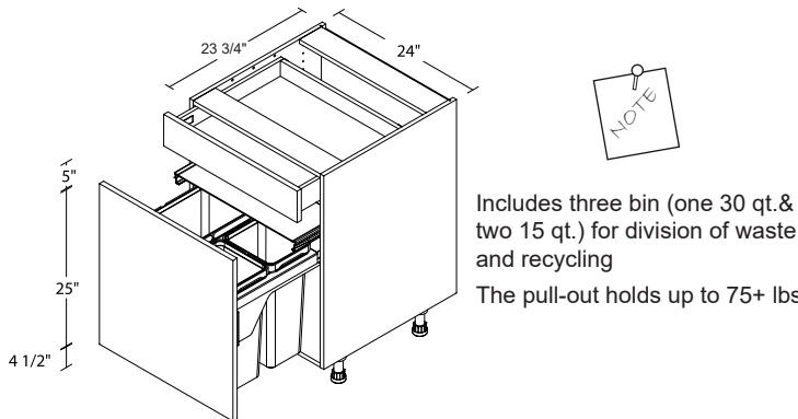
BASE PULL-OUT WITH 3 WASTE BINS / 1 DRAWER 24" B24SWB
