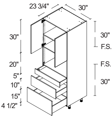
TALL MICROWAVE 1 / 2 DOORS / 3 DRAWERS
