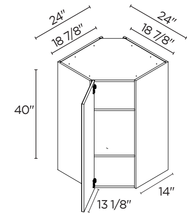
CORNER WALL 40" HIGH / 1 DOOR
