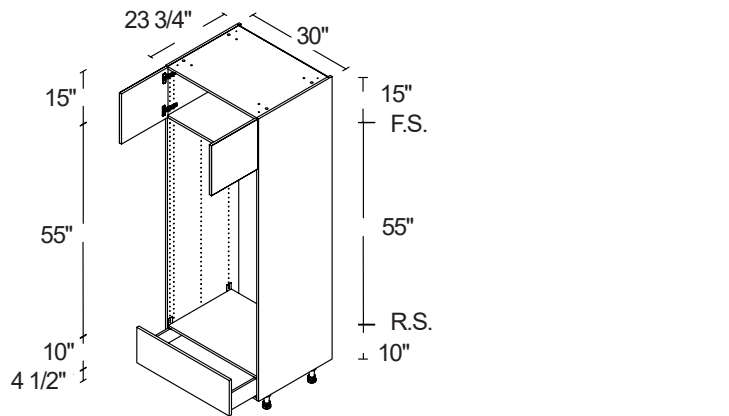
TALL DOUBLE OVEN 3 / 2 DOORS 1 DRAWER
