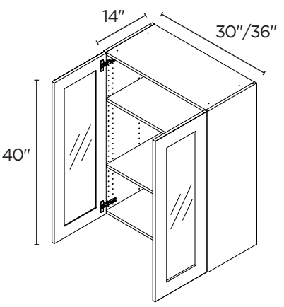
WALL 40" HIGH / 2 GLASS DOORS*
