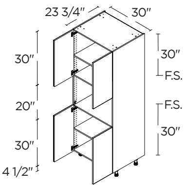
TALL MICROWAVE 1 / 4 DOORS
