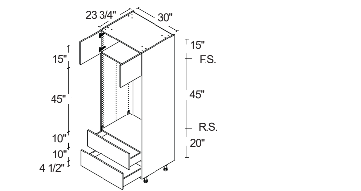
TALL MICRO / WALL OVEN 2 / 2 DOORS / 2 DRAWERS
