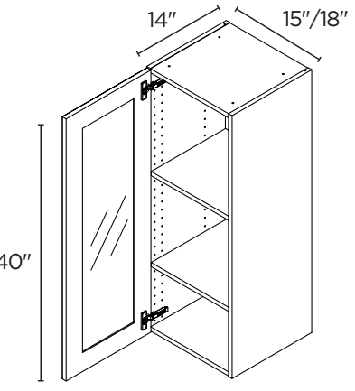
WALL 40" HIGH / 1 GLASS DOOR*
