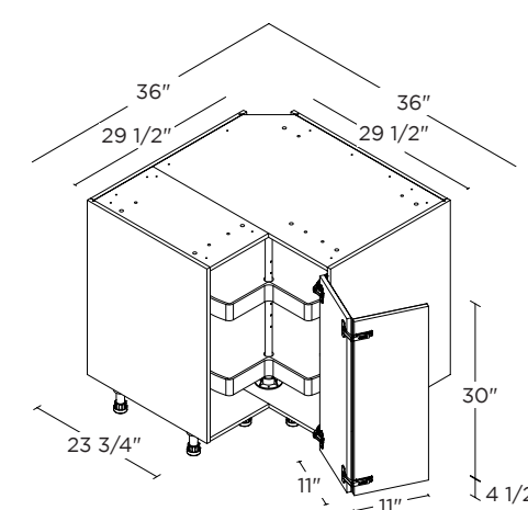
CORNER BASE WITH PREMIUM LAZY SUSAN 36" BC36LSP(L/R)
