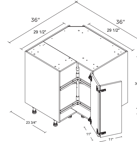
CORNER BASE WITH PREMIUM LAZY SUSAN 36" BC36LSP(L/R)
