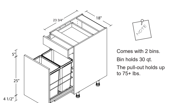
BASE PULL-OUT WITH 2 WASTE BINS / 1 DRAWER 18" B18SWB
